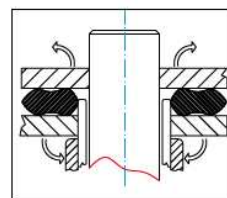
Dual contact sealed chain EXR1
