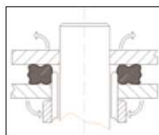
Dual contact sealed chain RDG
