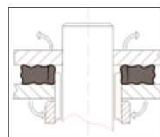
Triple contact sealed chain XTG - RTG1
