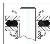
Dual contact sealed chain EXR1
