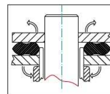
Dual contact sealed chain EXR1
