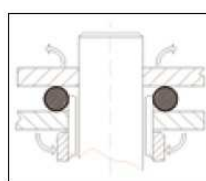
Standard sealed chain SSR
